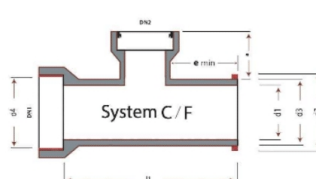
Normal Junction
