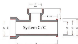
Compact Junction
